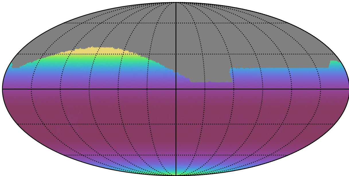
extra_ss_neo2_v3.4_10yrs All sky all bands: Min airmass
