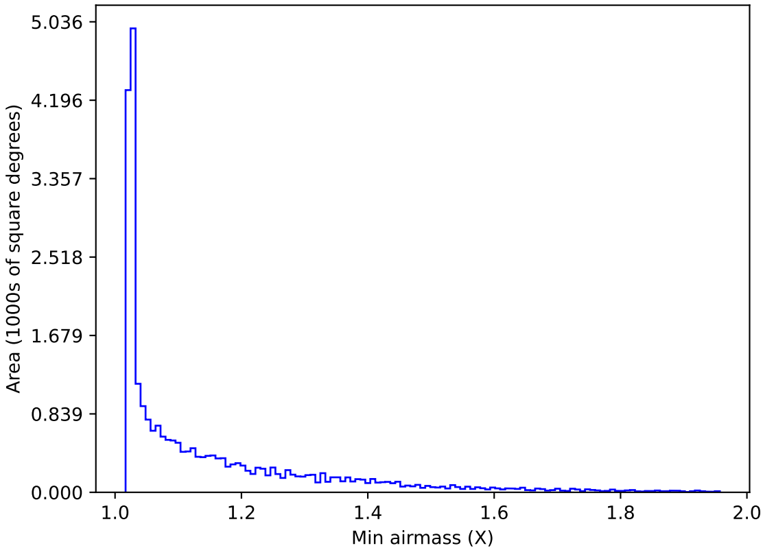
extra_ss_neo2_v3.4_10yrs All sky all bands: Min airmass
