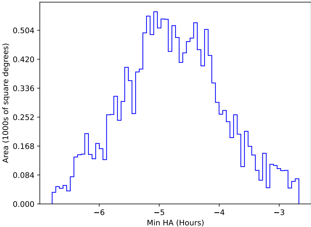
extra_ss_neo2_v3.4_10yrs WFD all bands: Min HA
