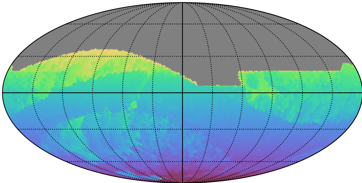
extra_ss_neo2_v3.4_10yrs All sky all bands: Min HA
