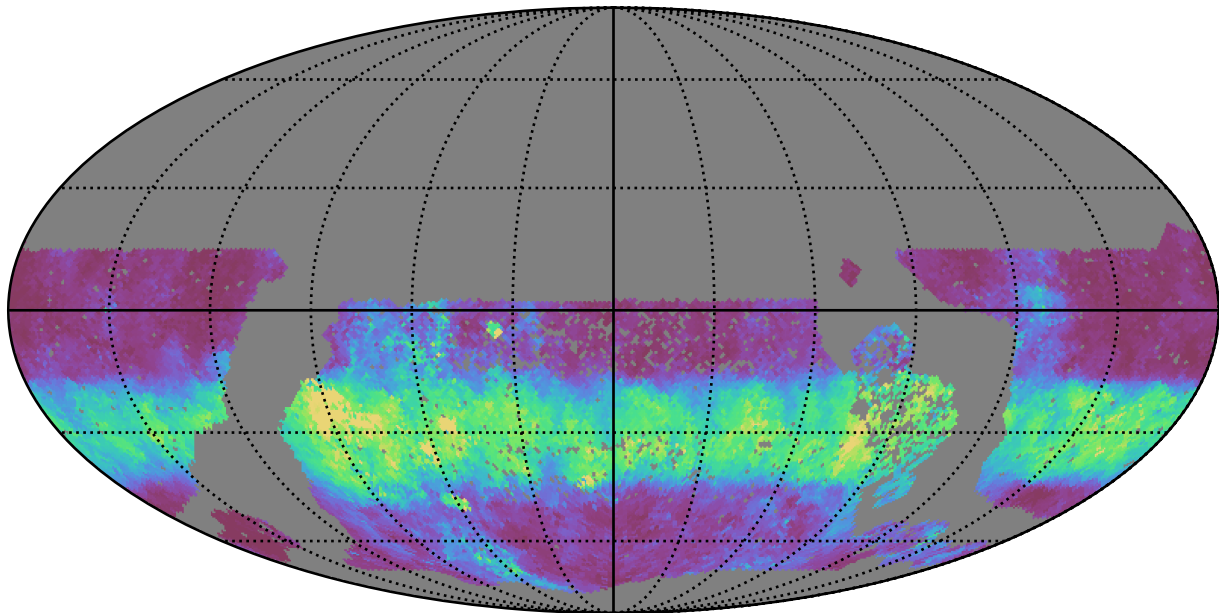
extra_ss_neo2_v3.4_10yrs WFD u band: Median normairmass
