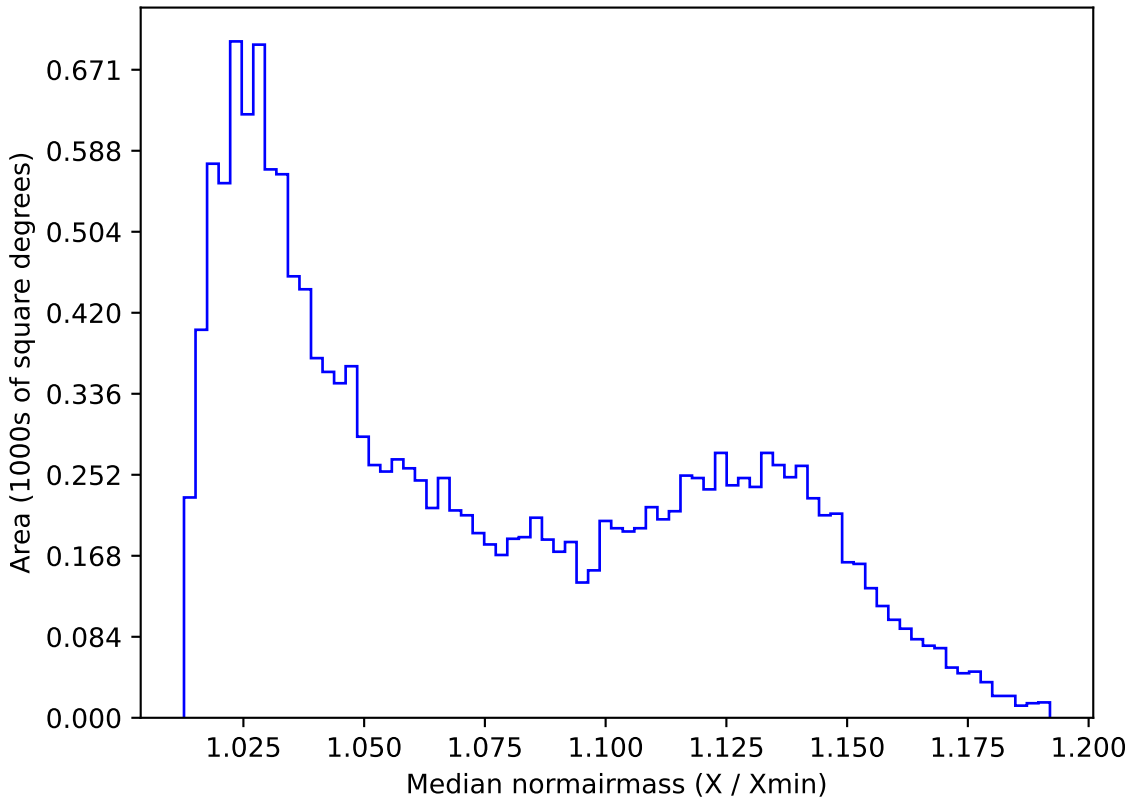
extra_ss_neo2_v3.4_10yrs WFD u band: Median normairmass
