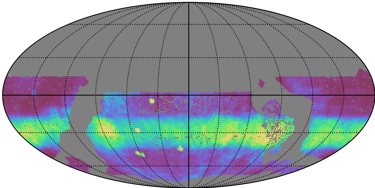
extra_ss_neo2_v3.4_10yrs WFD r band: Median normairmass
