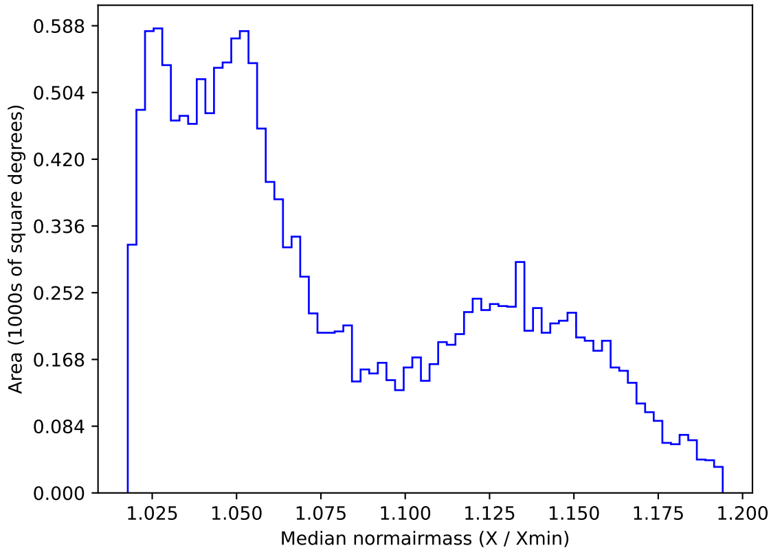
extra_ss_neo2_v3.4_10yrs WFD r band: Median normairmass
