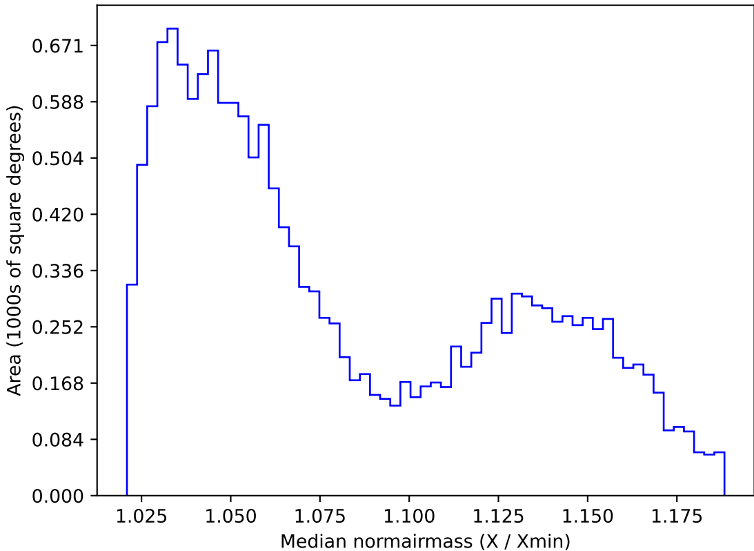
extra_ss_neo2_v3.4_10yrs WFD i band: Median normairmass
