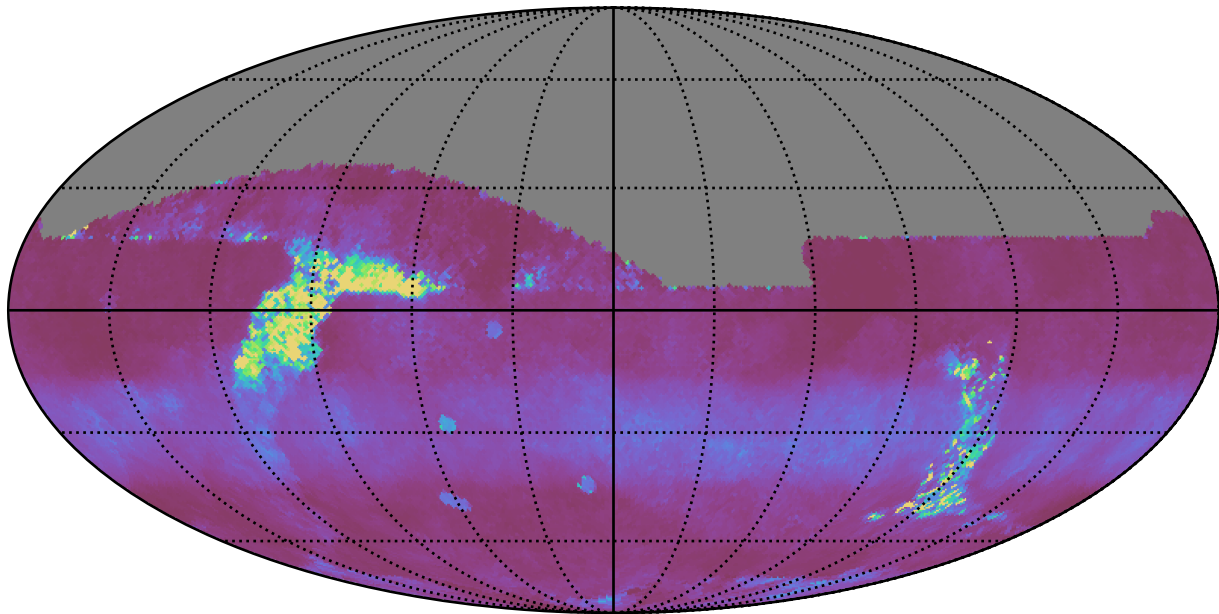
extra_ss_neo2_v3.4_10yrs All sky z band: Median normairmass
