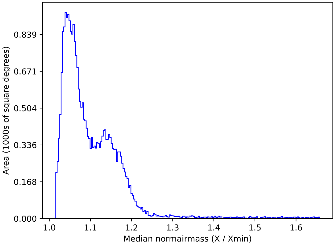
extra_ss_neo2_v3.4_10yrs All sky z band: Median normairmass
