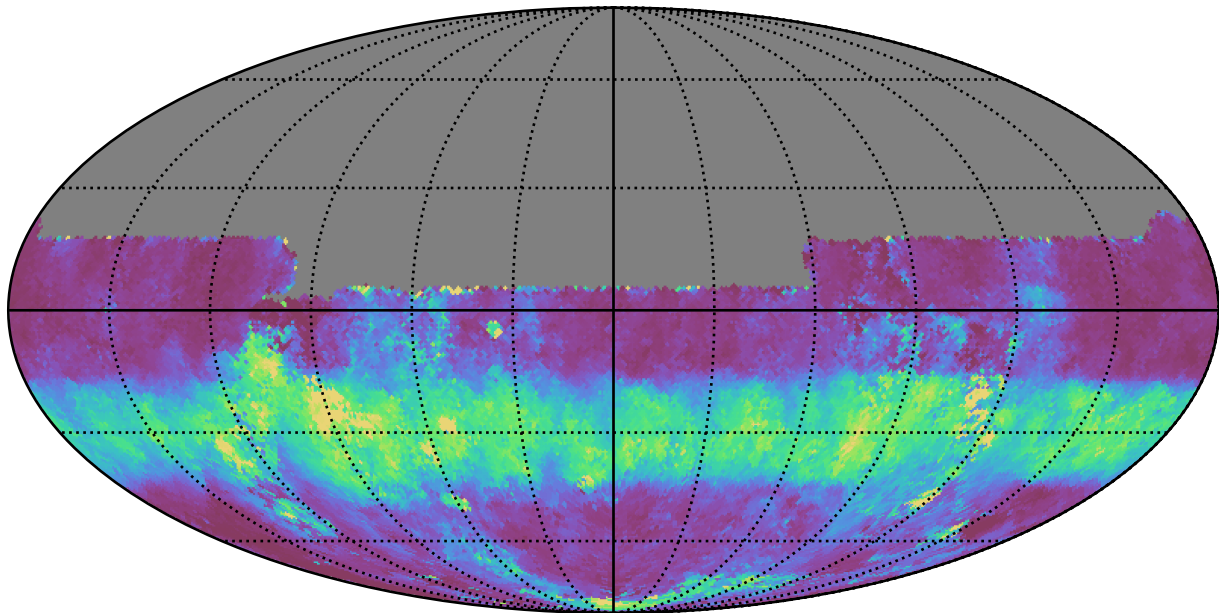
extra_ss_neo2_v3.4_10yrs All sky u band: Median normairmass
