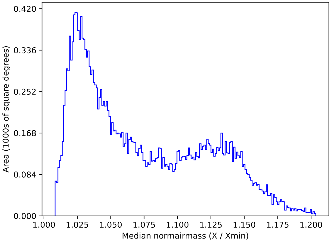
extra_ss_neo2_v3.4_10yrs All sky u band: Median normairmass
