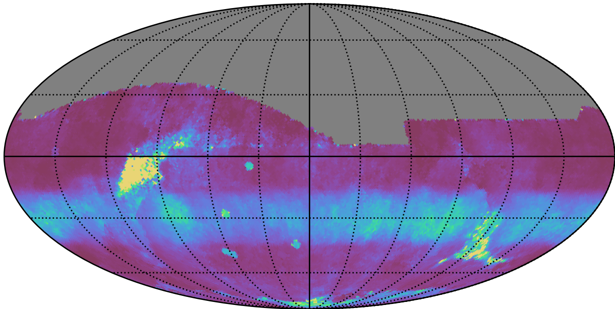
extra_ss_neo2_v3.4_10yrs All sky r band: Median normairmass
