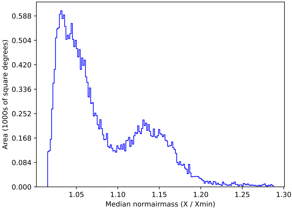
extra_ss_neo2_v3.4_10yrs All sky i band: Median normairmass
