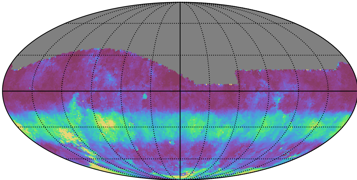
extra_ss_neo2_v3.4_10yrs All sky g band: Median normairmass
