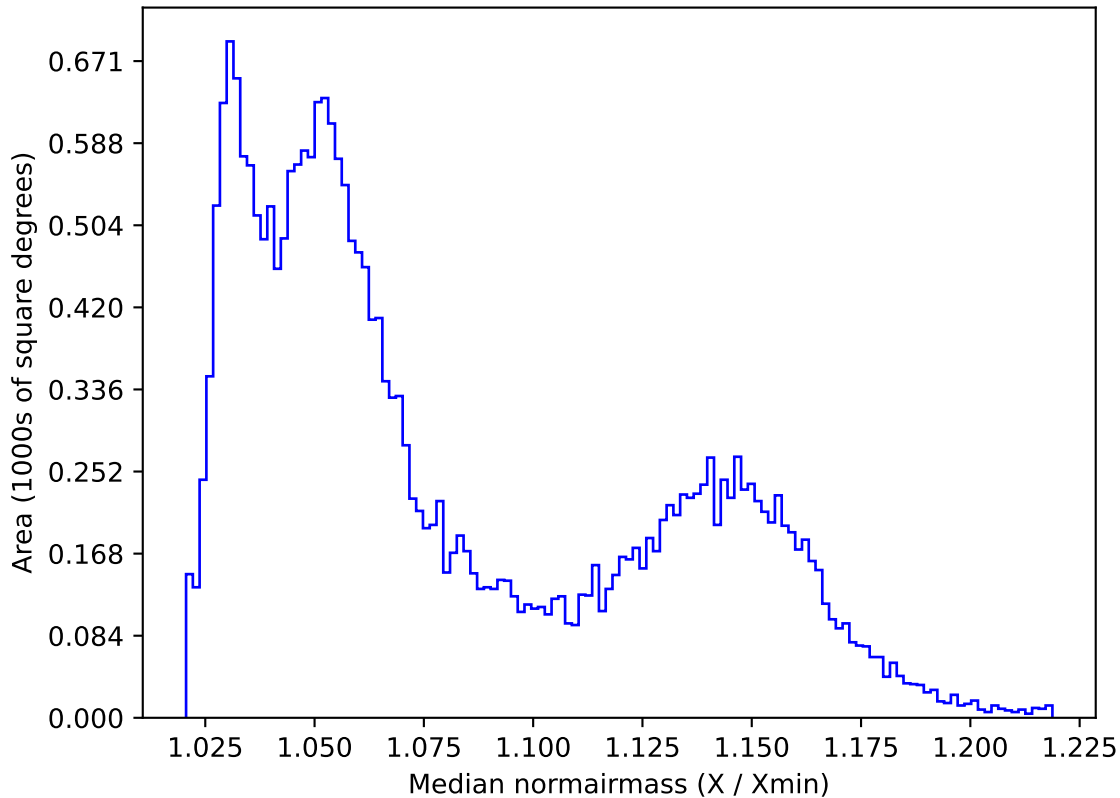
extra_ss_neo2_v3.4_10yrs All sky all bands: Median normairmass
