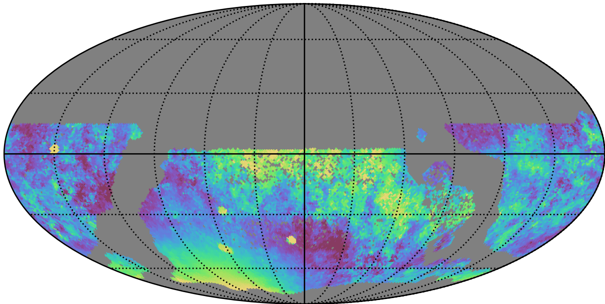
extra_ss_neo2_v3.4_10yrs WFD z band: Median moonDistance
