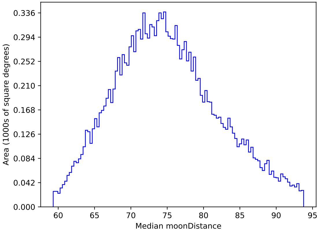
extra_ss_neo2_v3.4_10yrs WFD z band: Median moonDistance
