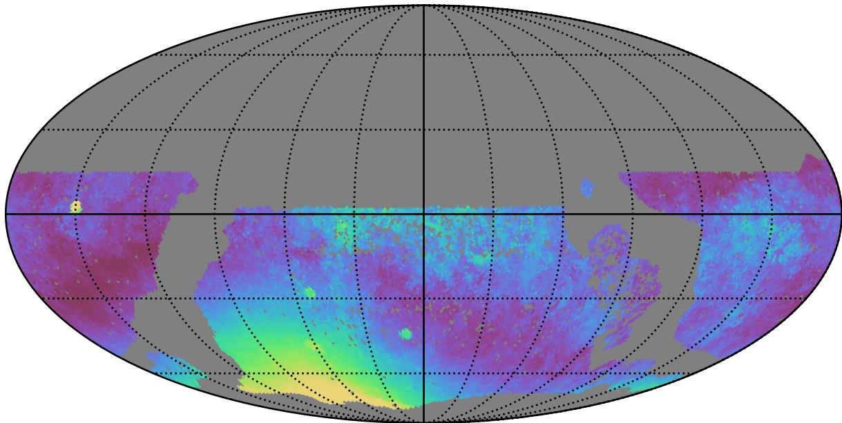
extra_ss_neo2_v3.4_10yrs WFD y band: Median moonDistance
