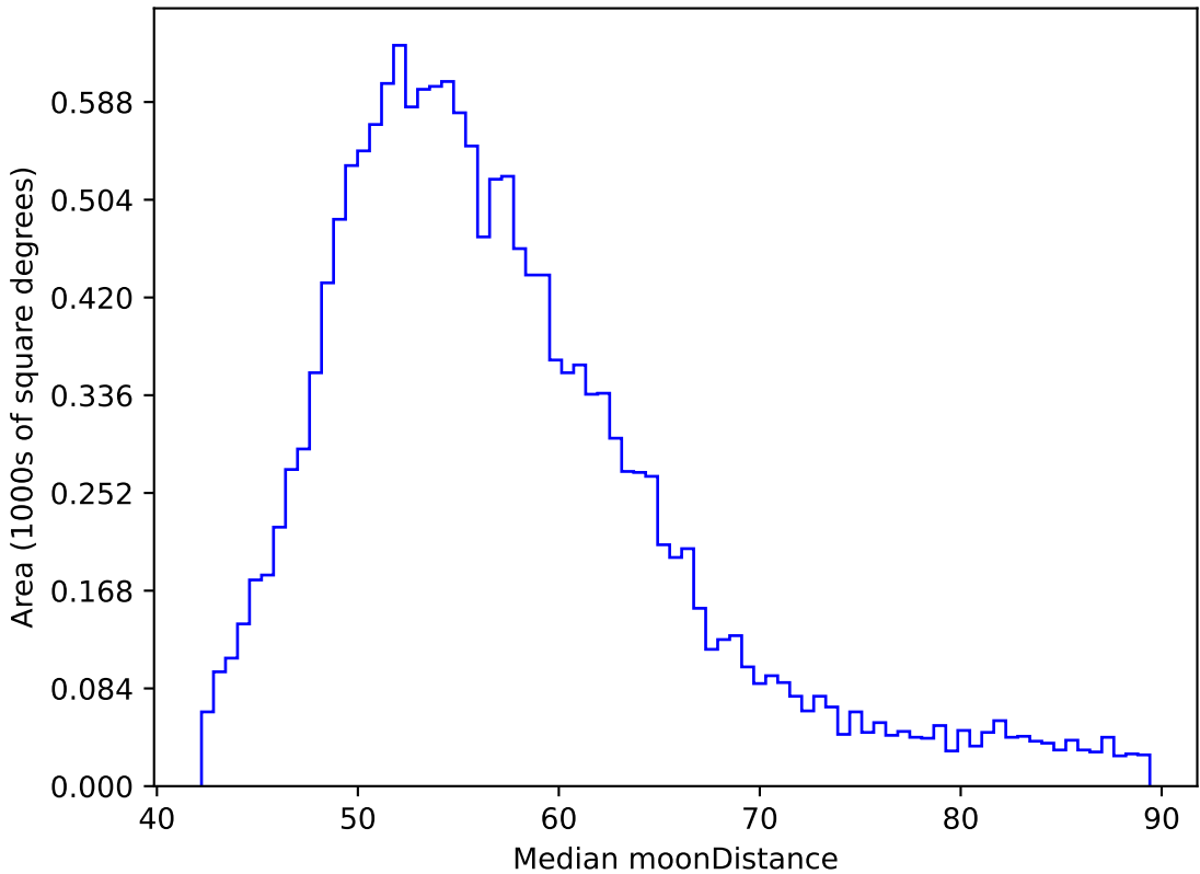
extra_ss_neo2_v3.4_10yrs WFD y band: Median moonDistance
