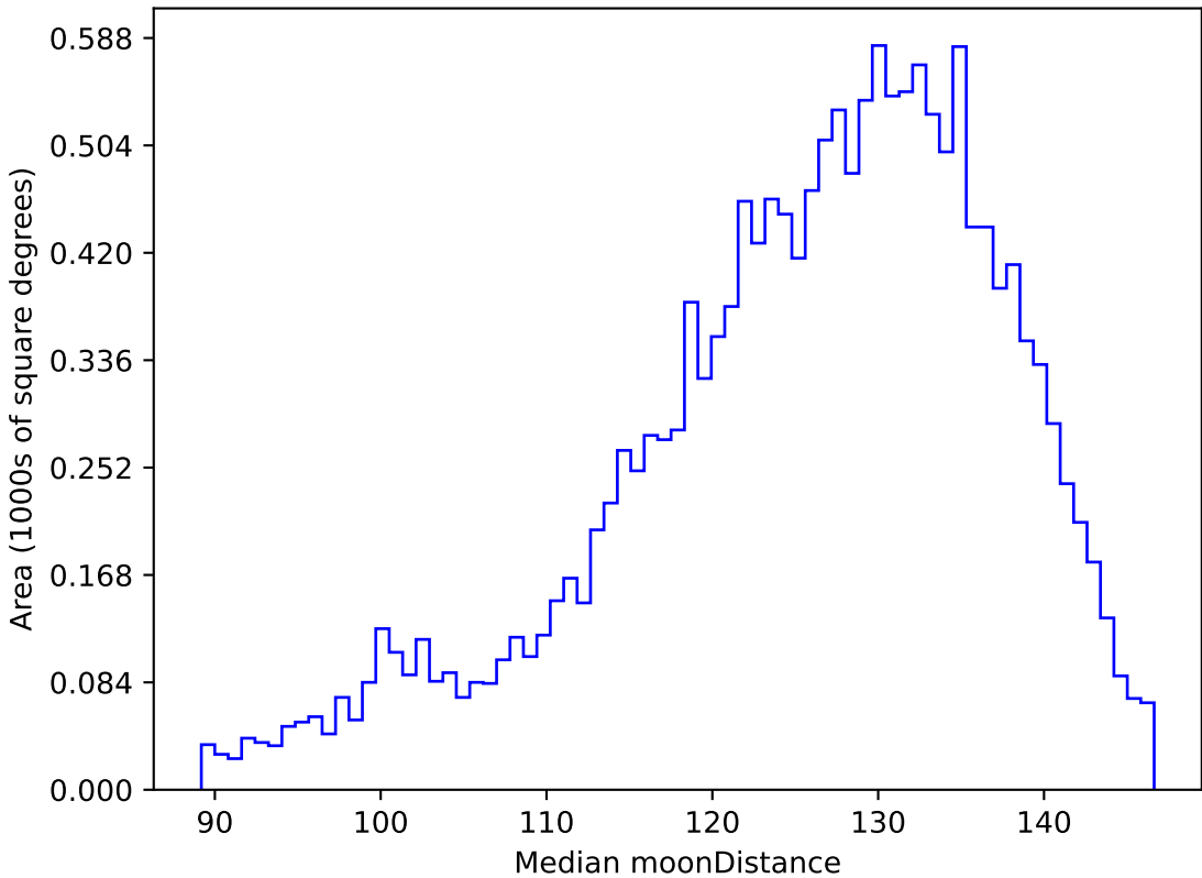
extra_ss_neo2_v3.4_10yrs WFD u band: Median moonDistance
