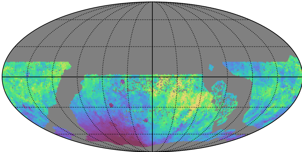
extra_ss_neo2_v3.4_10yrs WFD r band: Median moonDistance
