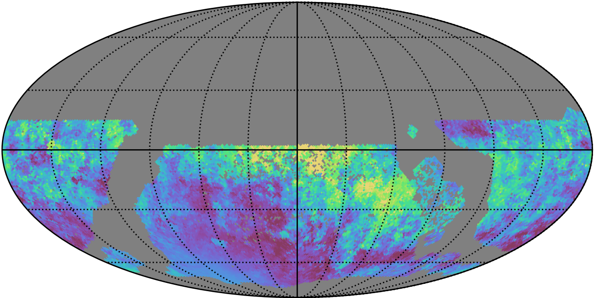
extra_ss_neo2_v3.4_10yrs WFD i band: Median moonDistance
