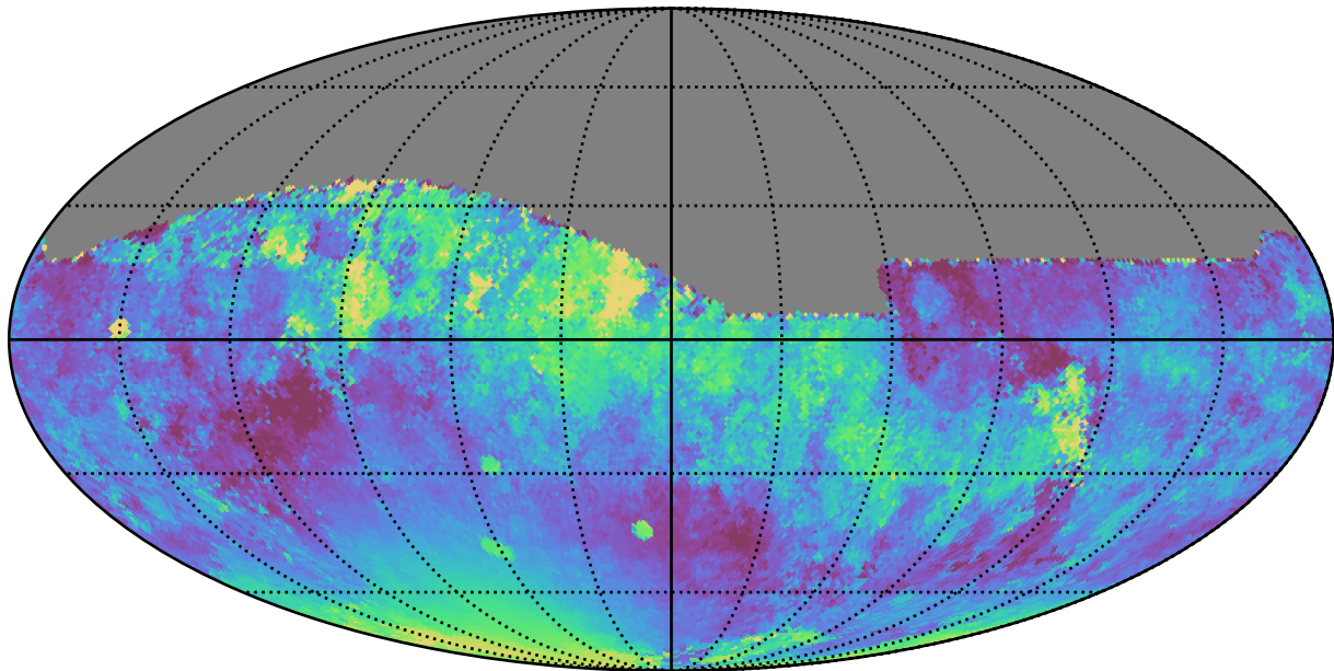
extra_ss_neo2_v3.4_10yrs All sky z band: Median moonDistance
