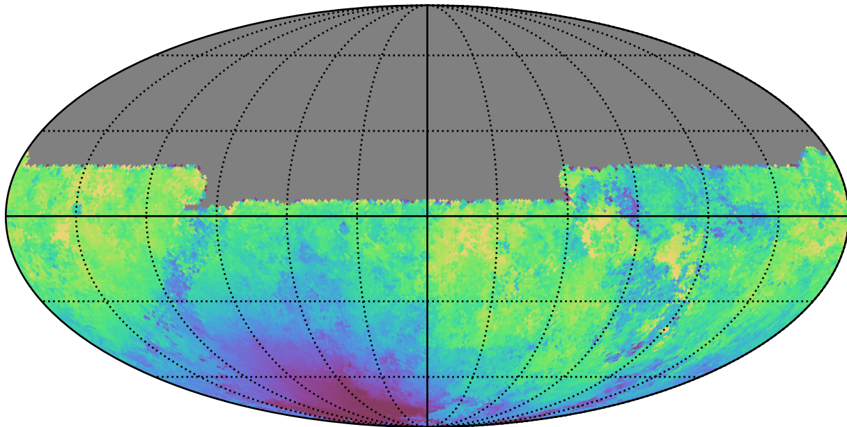
extra_ss_neo2_v3.4_10yrs All sky u band: Median moonDistance
