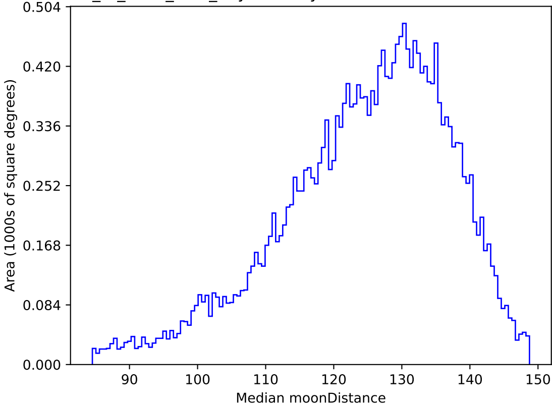
extra_ss_neo2_v3.4_10yrs All sky u band: Median moonDistance
