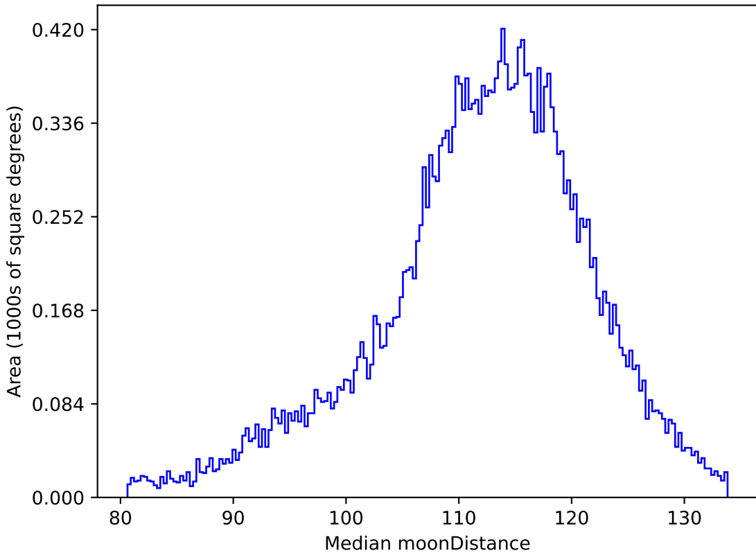
extra_ss_neo2_v3.4_10yrs All sky r band: Median moonDistance
