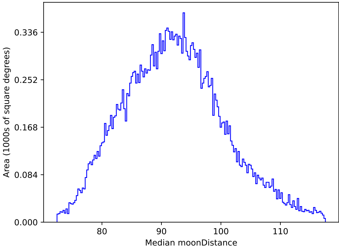
extra_ss_neo2_v3.4_10yrs All sky i band: Median moonDistance
