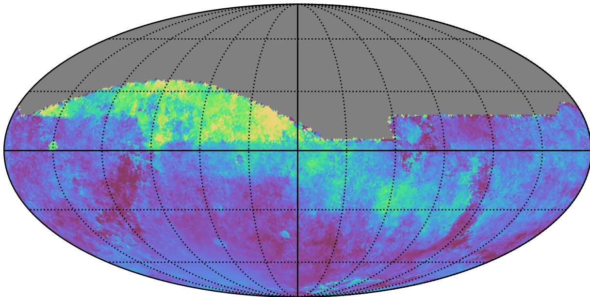
extra_ss_neo2_v3.4_10yrs All sky all bands: Median moonDistance
