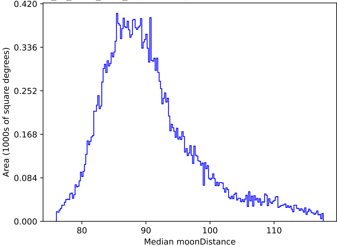
extra_ss_neo2_v3.4_10yrs All sky all bands: Median moonDistance
