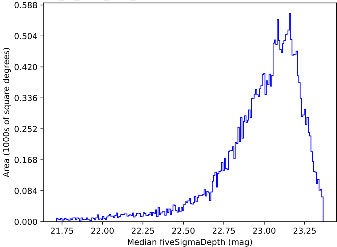
extra_ss_neo2_v3.4_10yrs Yr 1 z band: Median fiveSigmaDepth
