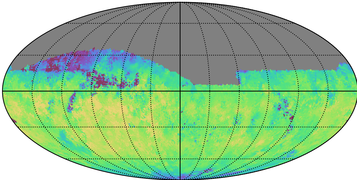
extra_ss_neo2_v3.4_10yrs Yr 1 i band: Median fiveSigmaDepth
