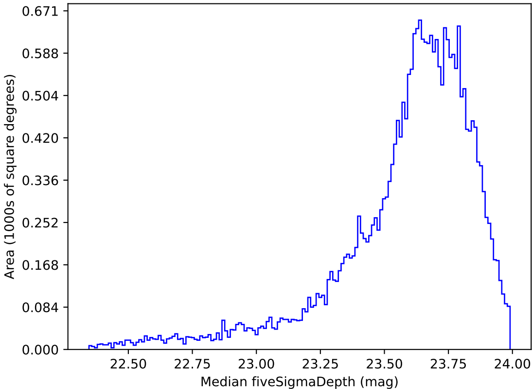
extra_ss_neo2_v3.4_10yrs Yr 1 i band: Median fiveSigmaDepth
