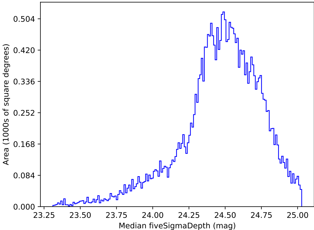
extra_ss_neo2_v3.4_10yrs Yr 1 g band: Median fiveSigmaDepth
