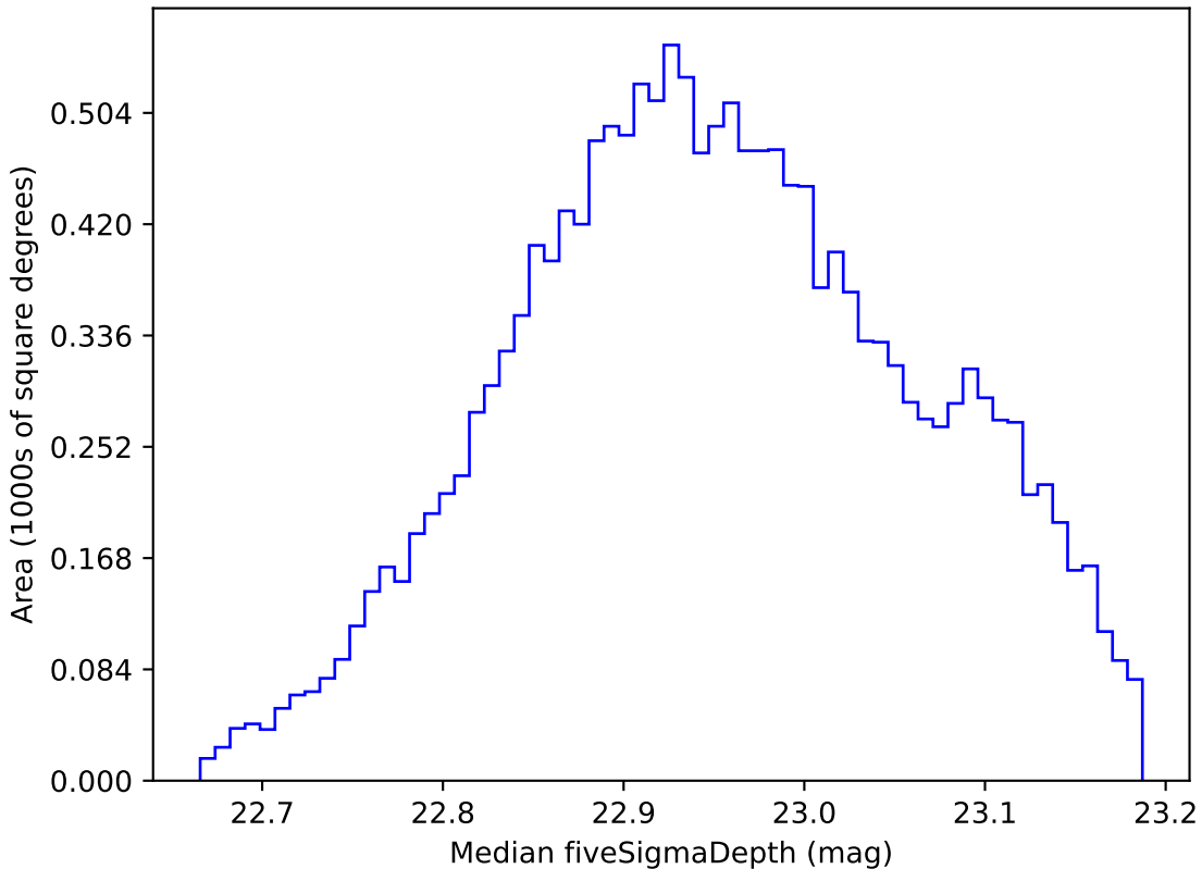
extra_ss_neo2_v3.4_10yrs WFD z band: Median fiveSigmaDepth
