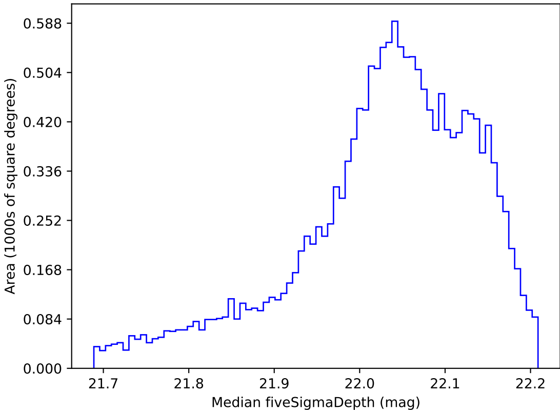
extra_ss_neo2_v3.4_10yrs WFD y band: Median fiveSigmaDepth
