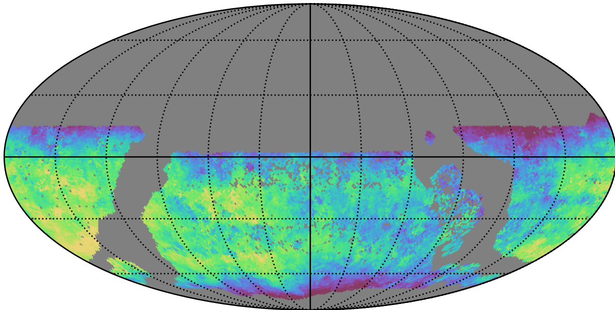
extra_ss_neo2_v3.4_10yrs WFD u band: Median fiveSigmaDepth
