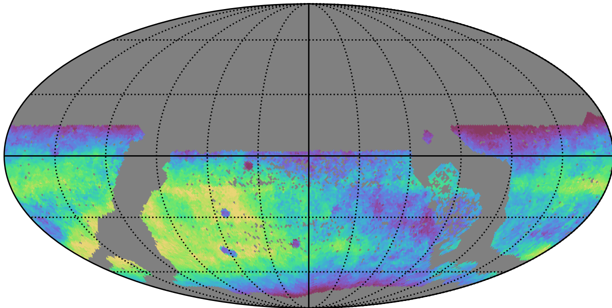
extra_ss_neo2_v3.4_10yrs WFD r band: Median fiveSigmaDepth
