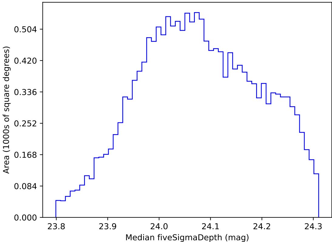
extra_ss_neo2_v3.4_10yrs WFD r band: Median fiveSigmaDepth
