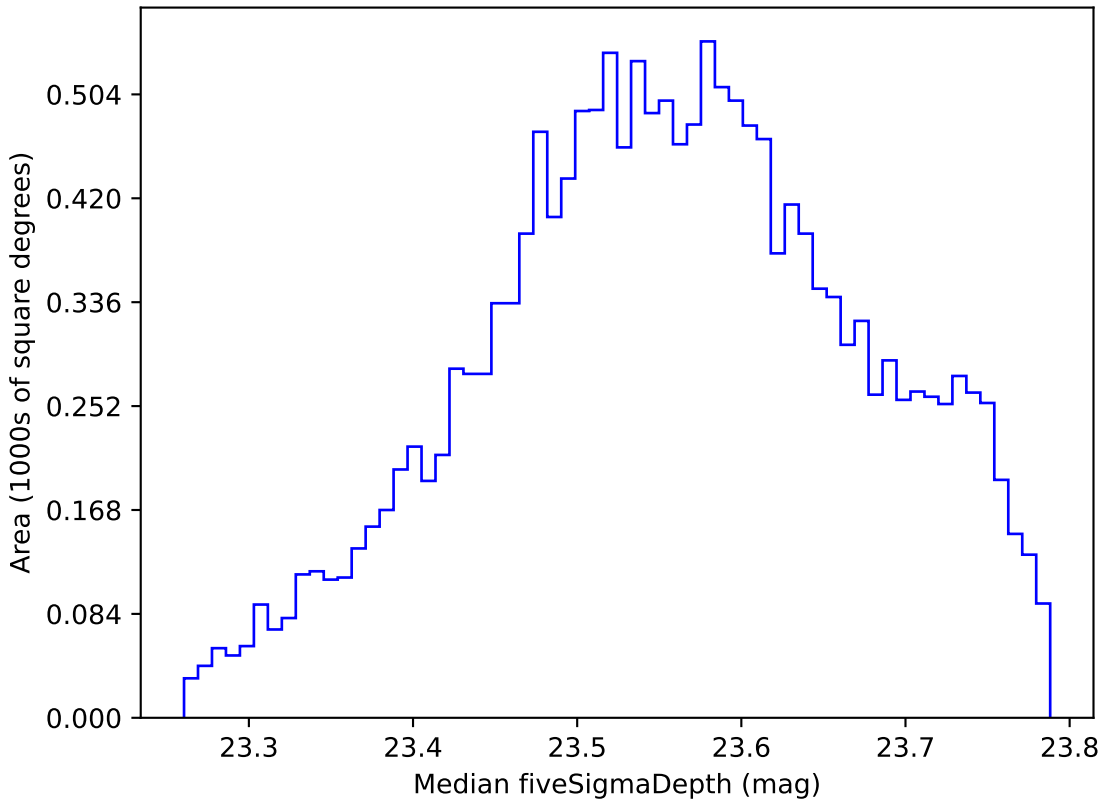
extra_ss_neo2_v3.4_10yrs WFD i band: Median fiveSigmaDepth
