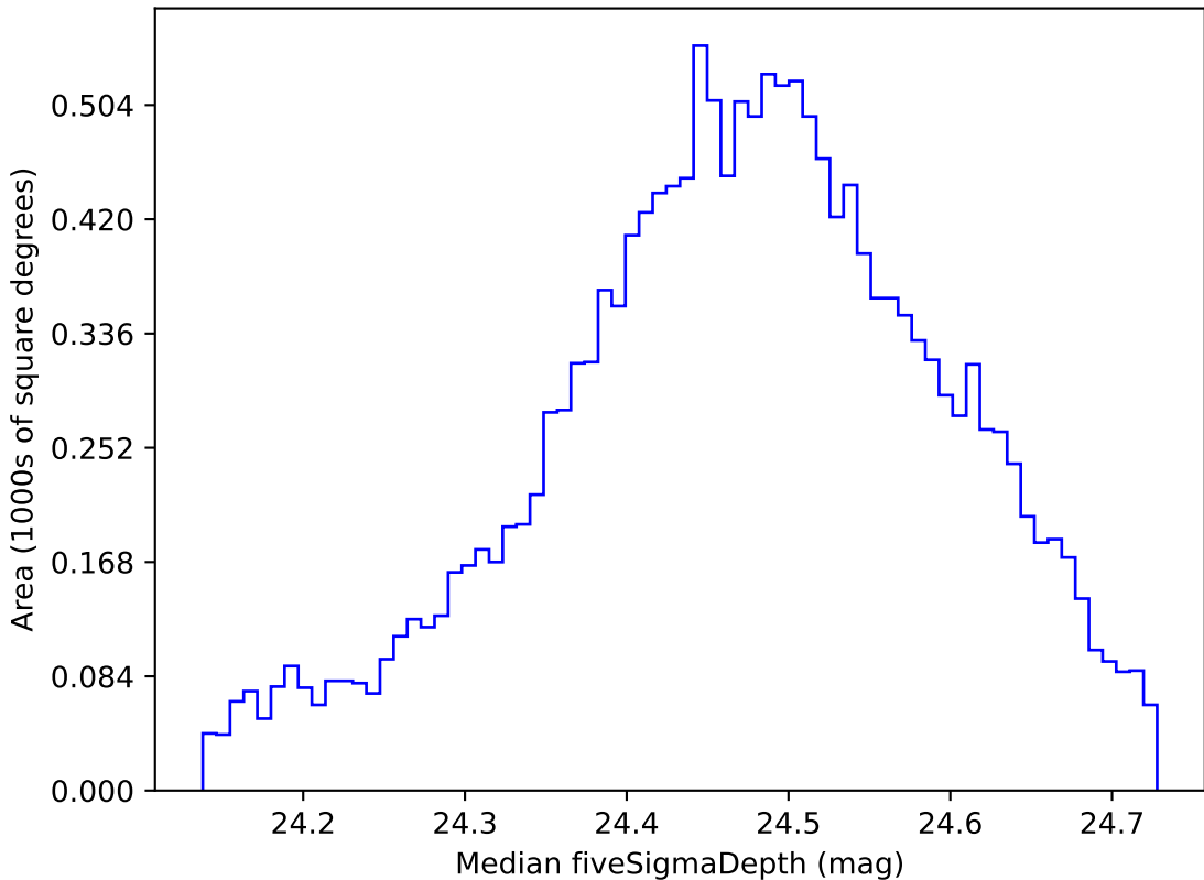
extra_ss_neo2_v3.4_10yrs WFD g band: Median fiveSigmaDepth
