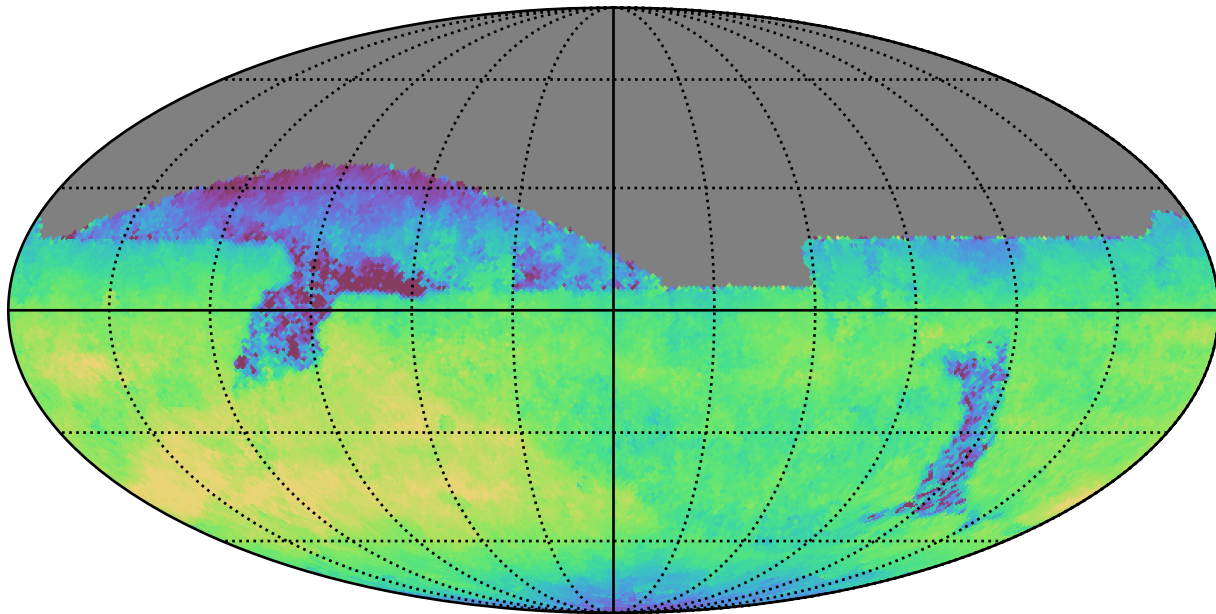
extra_ss_neo2_v3.4_10yrs All sky z band: Median fiveSigmaDepth
