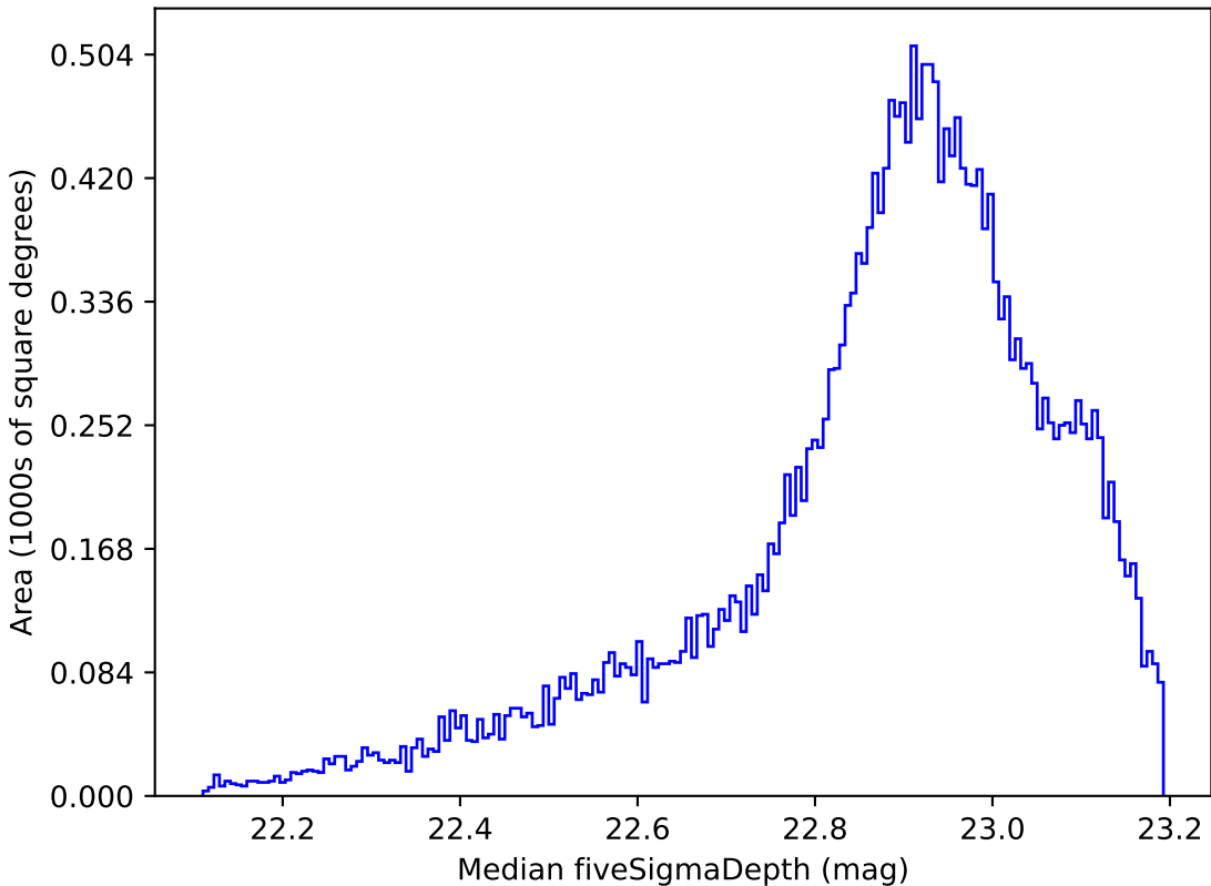
extra_ss_neo2_v3.4_10yrs All sky z band: Median fiveSigmaDepth
