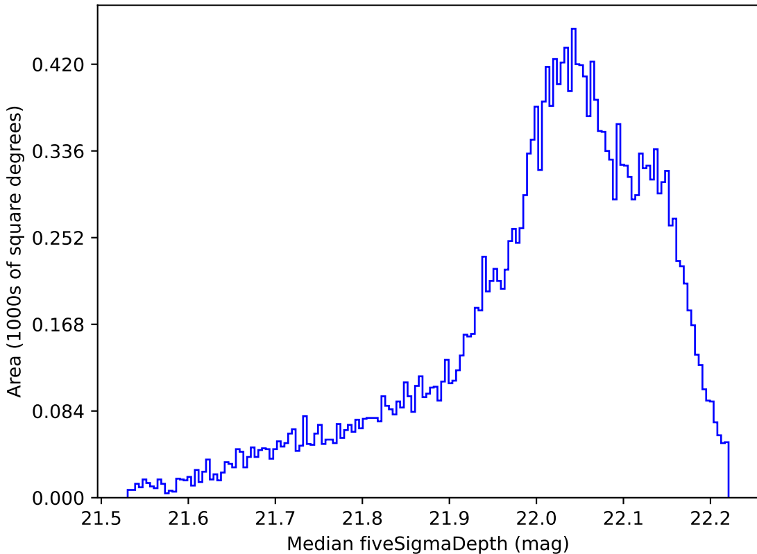
extra_ss_neo2_v3.4_10yrs All sky y band: Median fiveSigmaDepth
