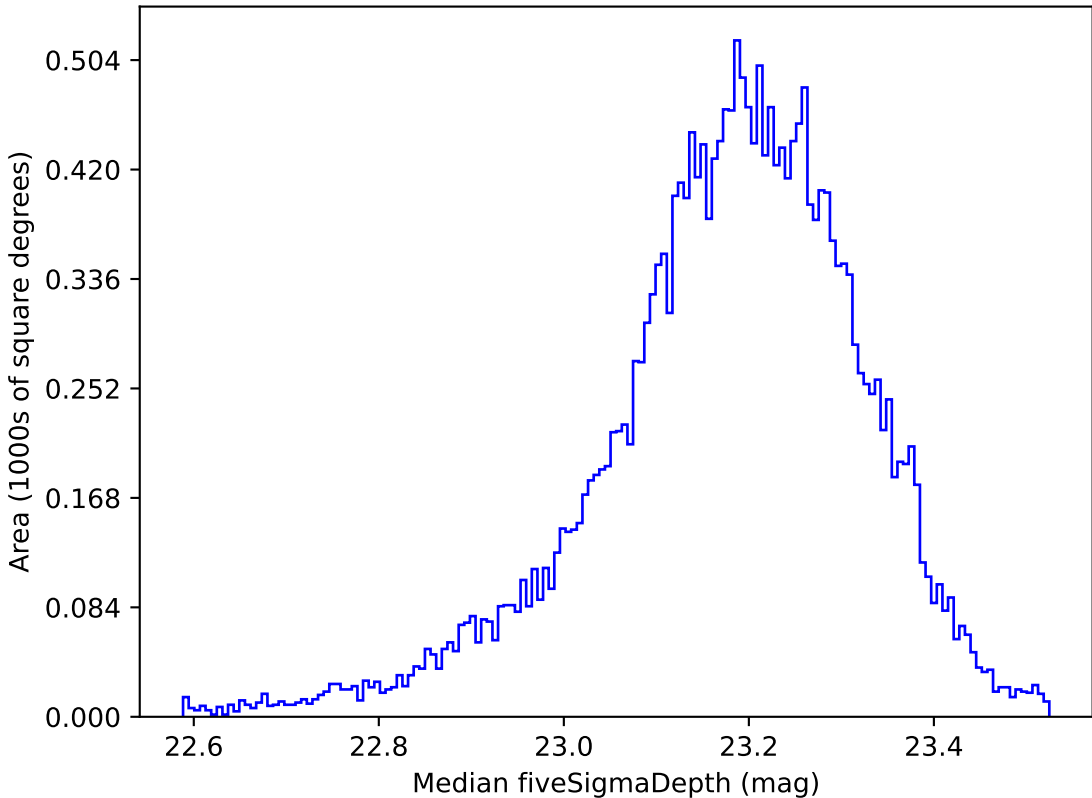
extra_ss_neo2_v3.4_10yrs All sky u band: Median fiveSigmaDepth
