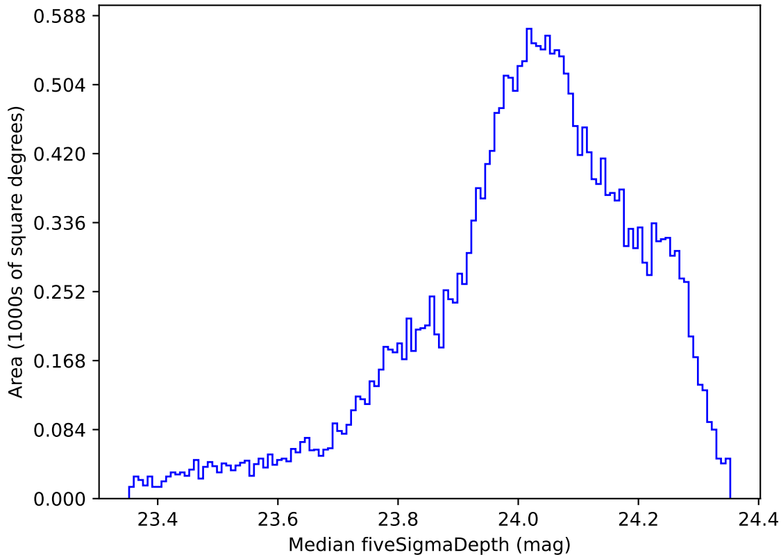
extra_ss_neo2_v3.4_10yrs All sky r band: Median fiveSigmaDepth
