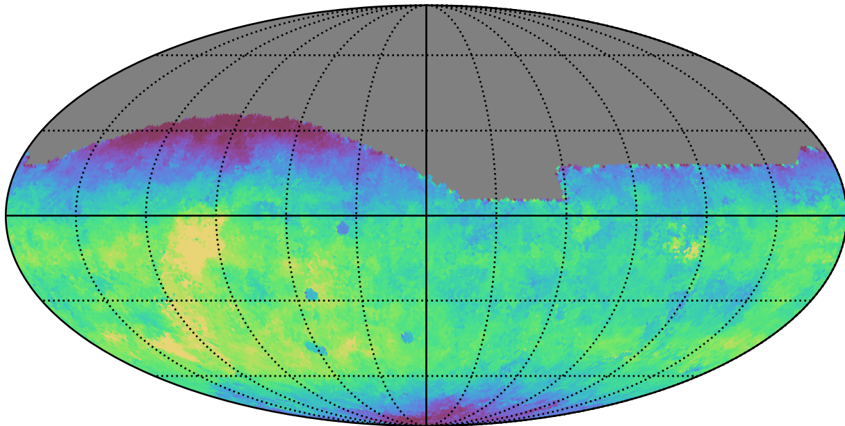
extra_ss_neo2_v3.4_10yrs All sky g band: Median fiveSigmaDepth
