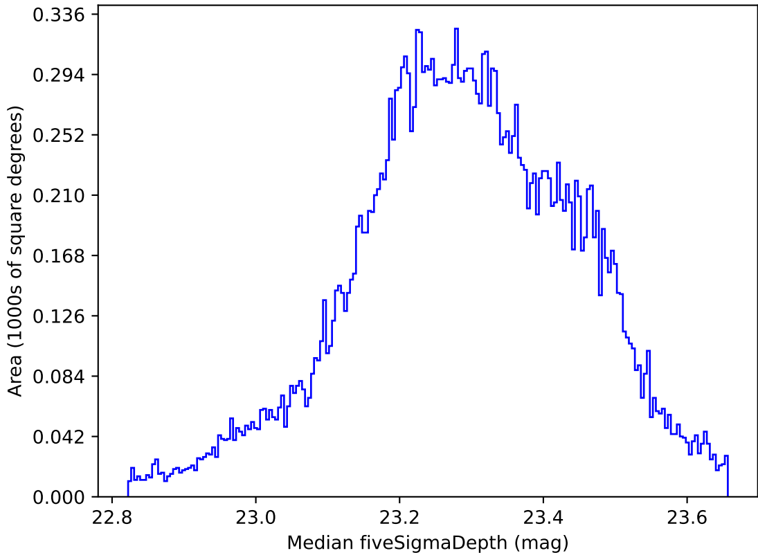
extra_ss_neo2_v3.4_10yrs All sky all bands: Median fiveSigmaDepth
