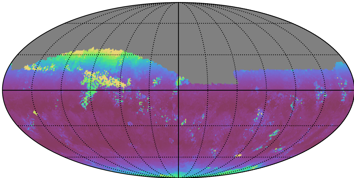
extra_ss_neo2_v3.4_10yrs Yr 1 z band: Median airmass
